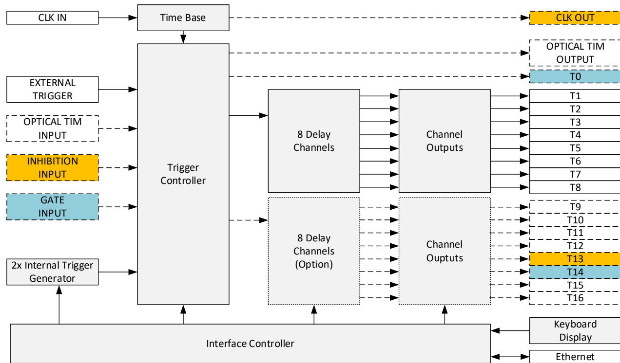
Block diagram of the delay generator (■ ■ ■ ■ only one input/output available)
