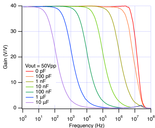
Frequency response for different capacitive loads
