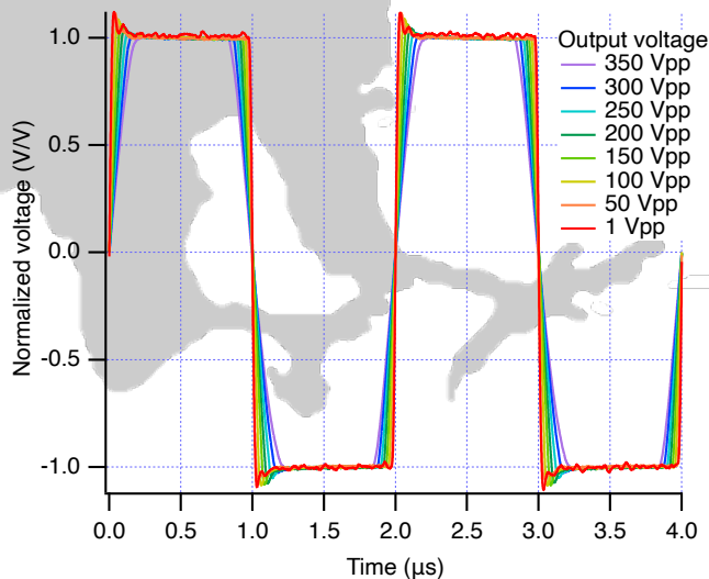
Step response
