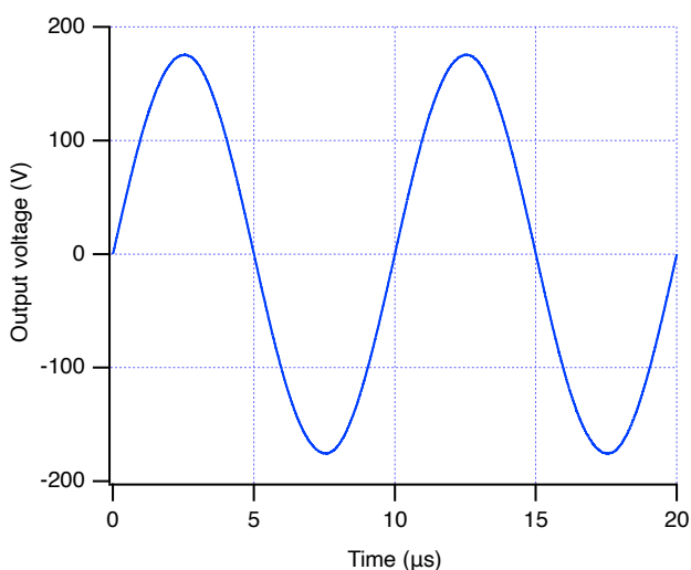
Sine wave full-swing output voltage response
