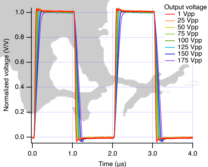
Step response
